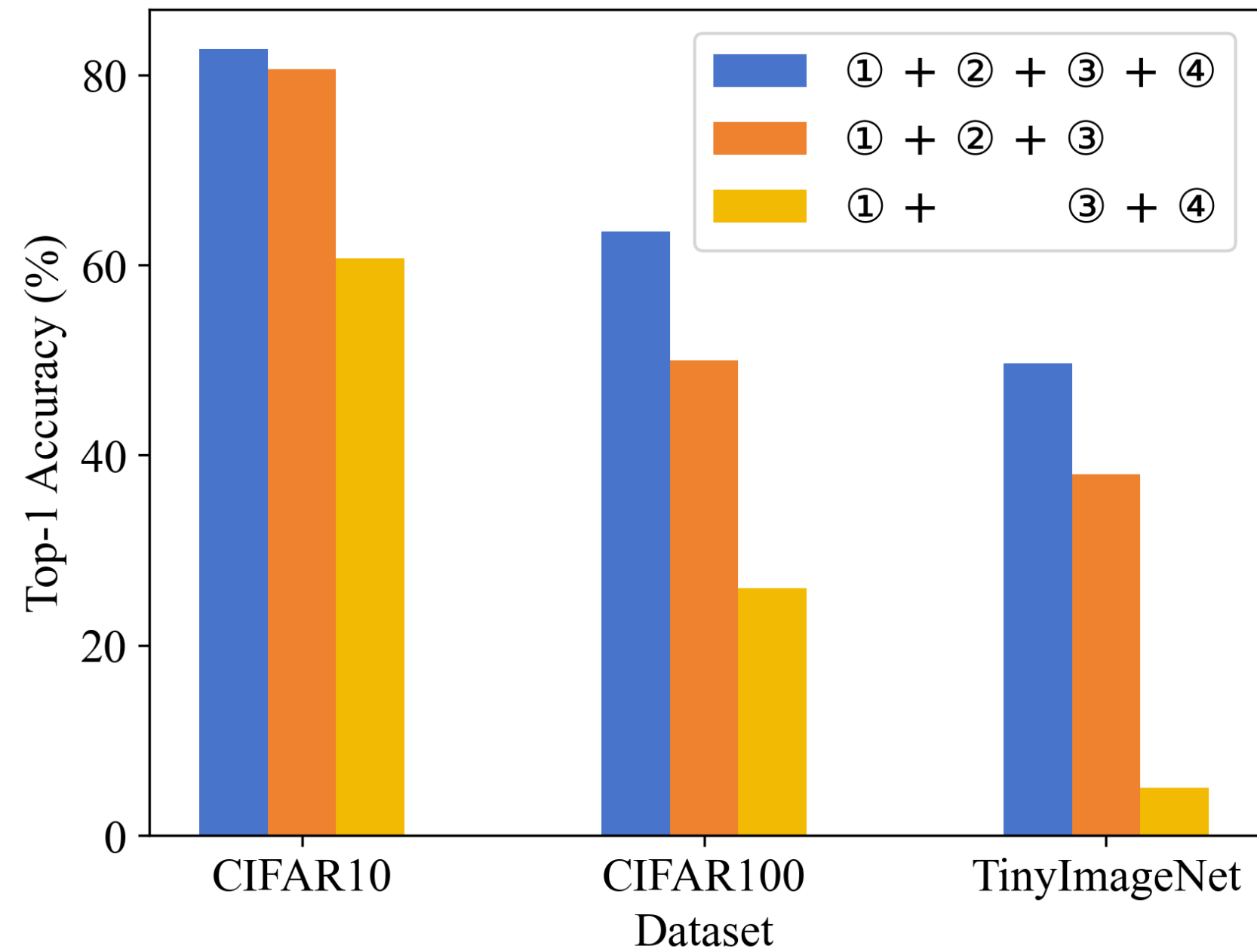
(c) Performance after removing skip connections
