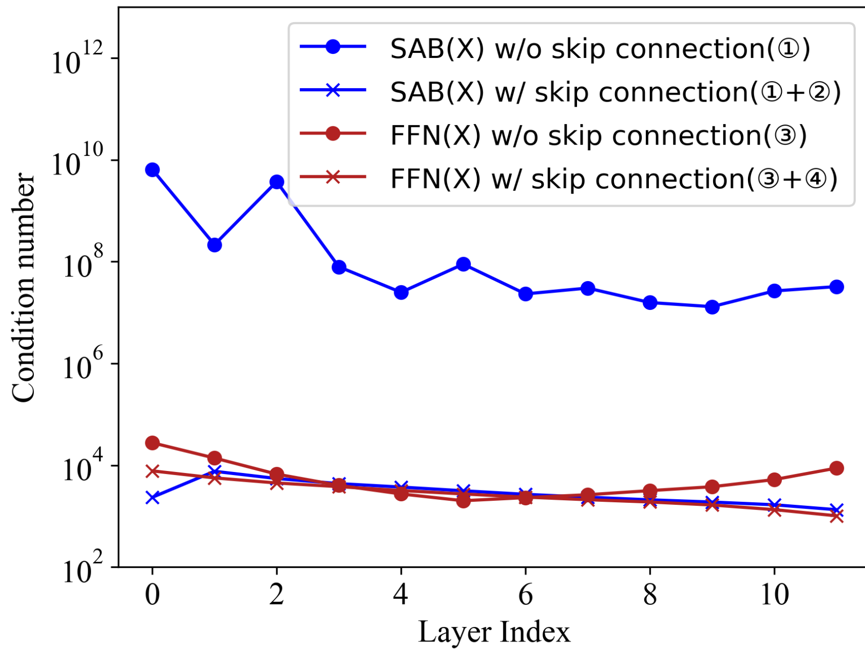
(b) FFN and SAB output condition number using different configurations
